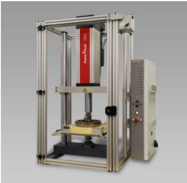
Dynamic fatigue test bench 5 kN
