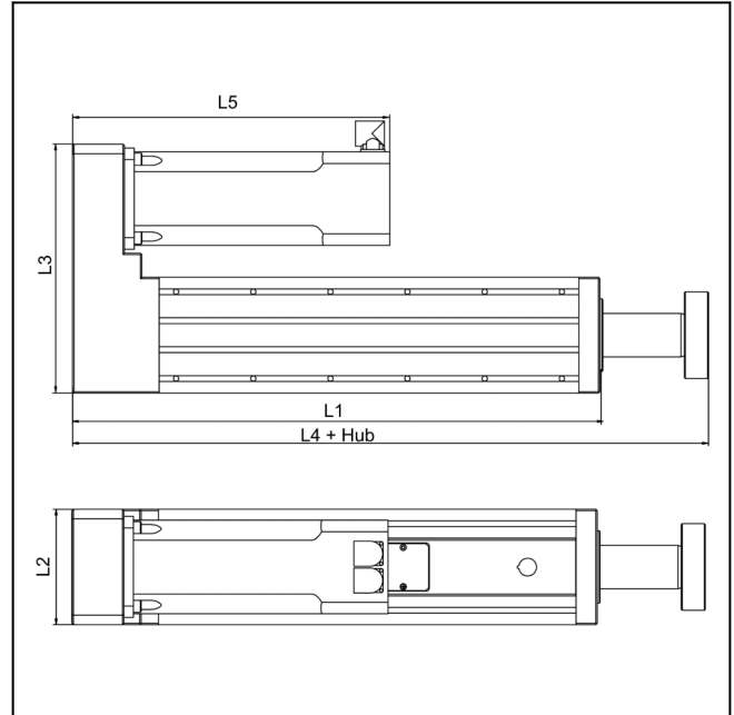
Drawing of elctro-mechanical testing actuator
