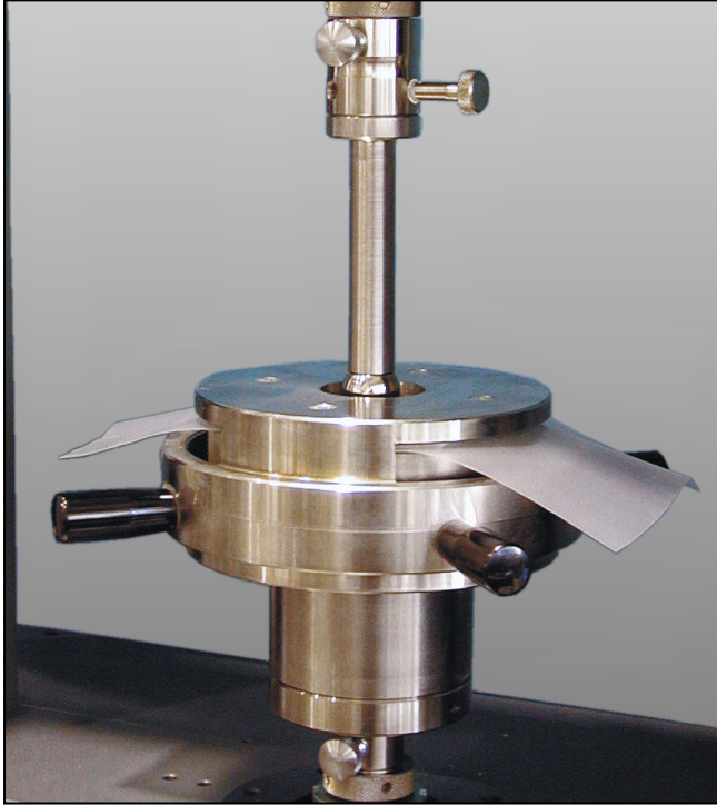
Ball burst test device
